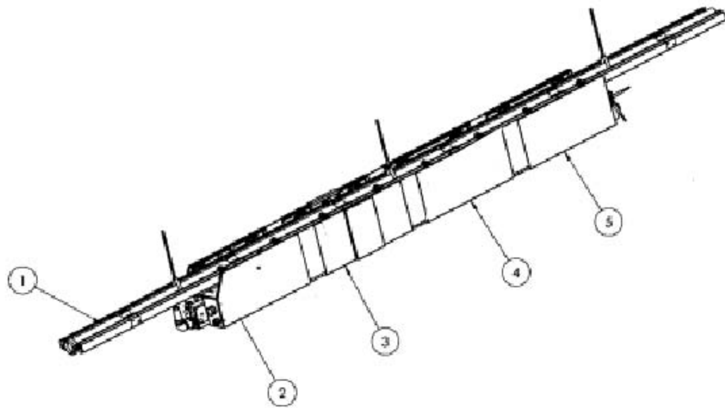
(1) Monorail; Mobile unit: (2) Control module; (3) Power module; (4) Drive module; (5) Fire-fighting module
